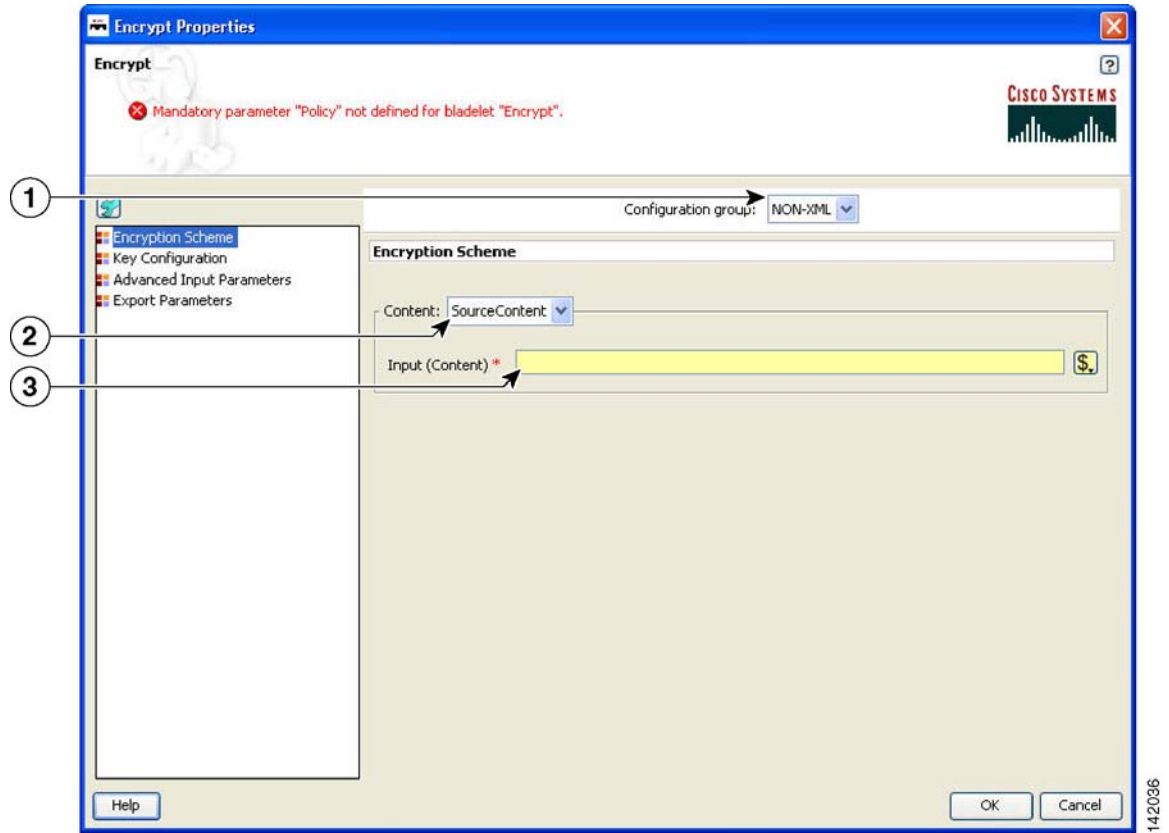
Figure 120 Encrypt Properties Window—Encryption Scheme, Non-XML, Source Content
