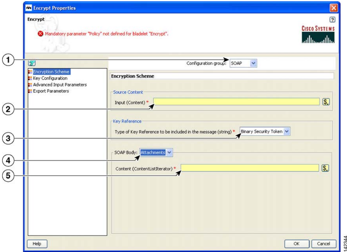
Figure 117 Encrypt Properties Window—Encryption Scheme, SOAP, Attachments
