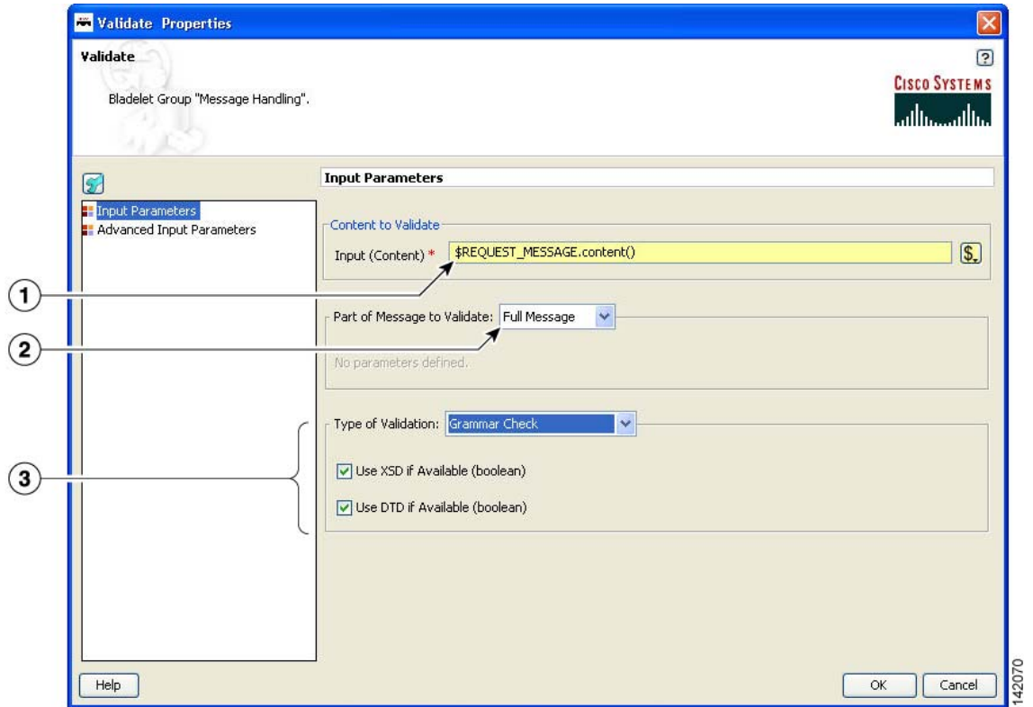
Figure 60 Validate Properties Window—Input Parameters, Validate
