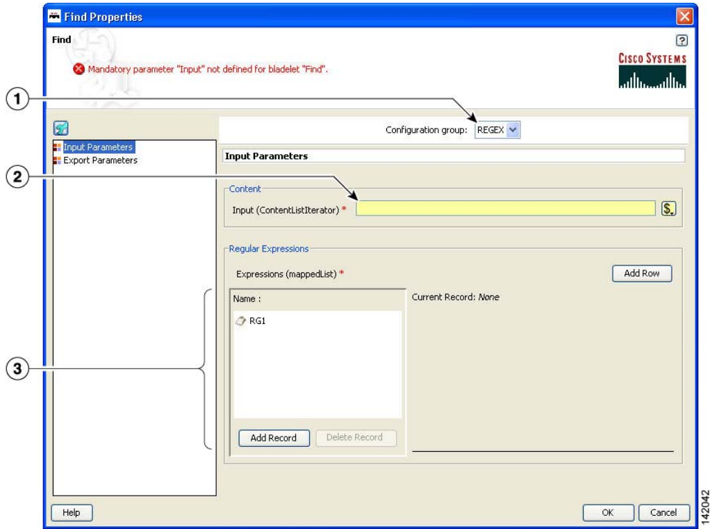
Figure 56 Find Properties Window—Input Parameters, Regex
