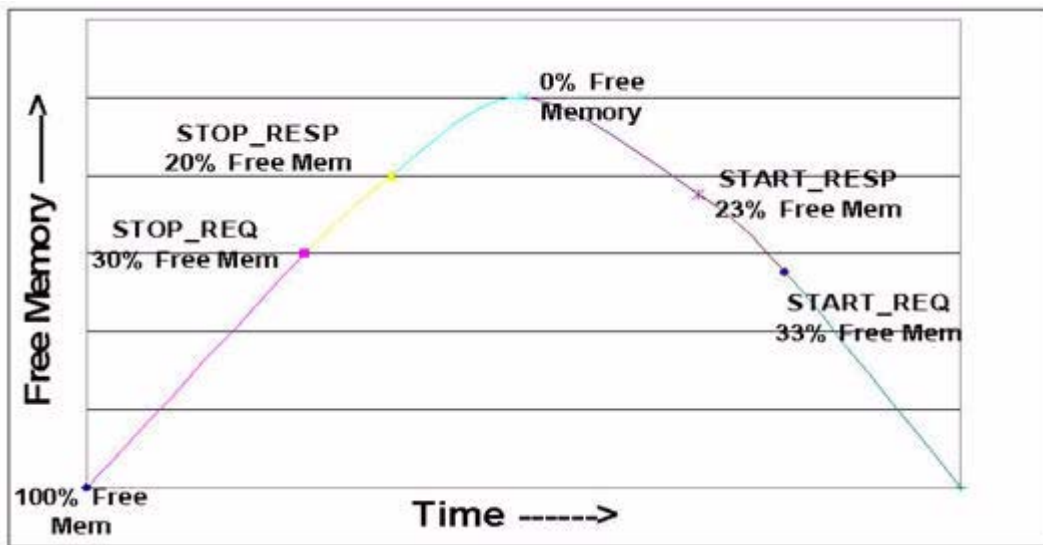
Figure 3-17 Graceful Handling Request and Response Thresholds
