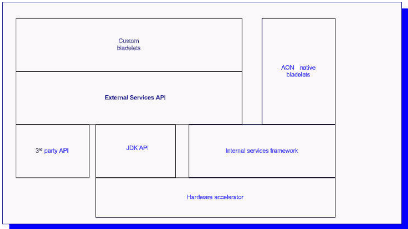
Figure 5-2 External Services Architecture
