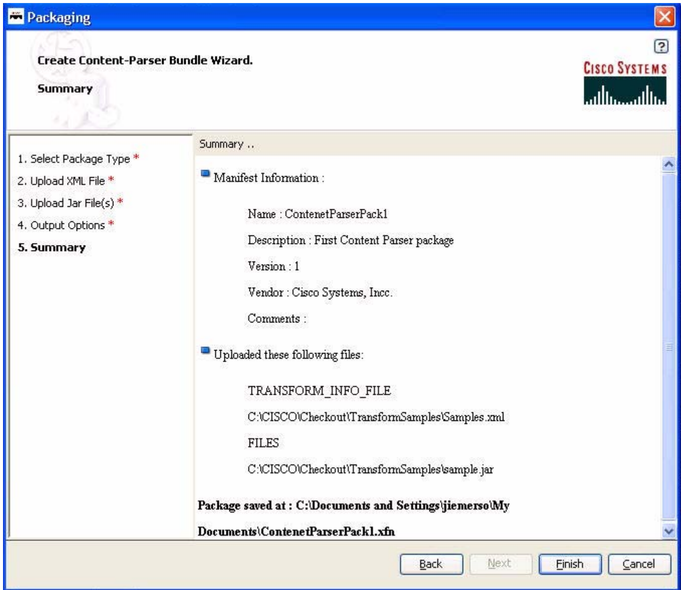
Figure 5-13 Content-Parser summary window
