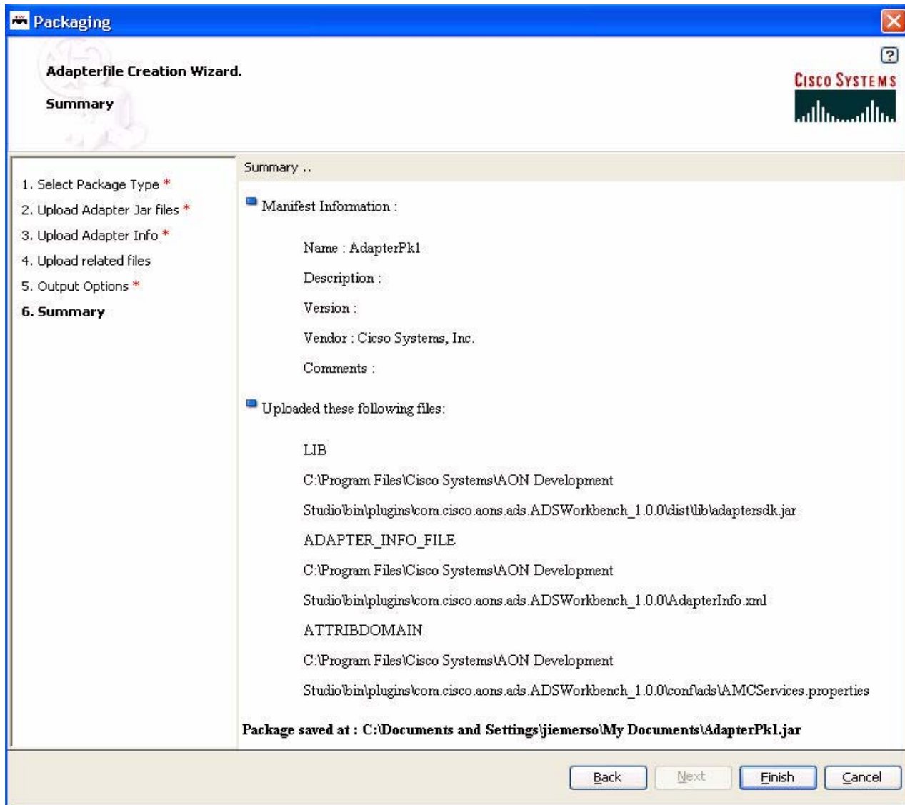
Figure 3-11 Adapterfile creation summary window
