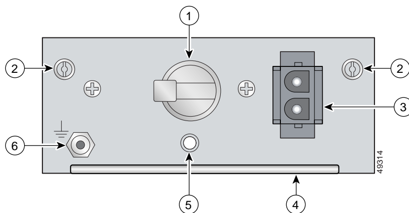
Figure 2 DC PEM Faceplate
