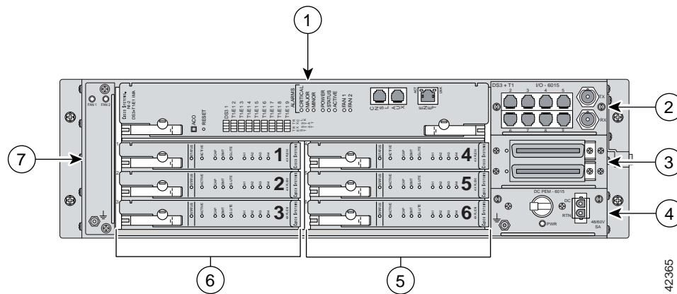
Figure 1 DC PEM Location in the Cisco 6015 Chassis
