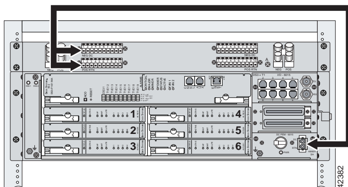
Figure 5 Connecting the DC PEM to the Fuse and Alarm Panel
