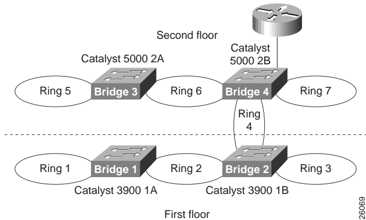
Figure 10-1 Initial Network Configuration
