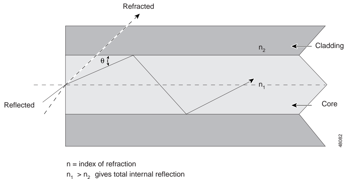
Figure 2-6 Principle of Total Internal Reflection
