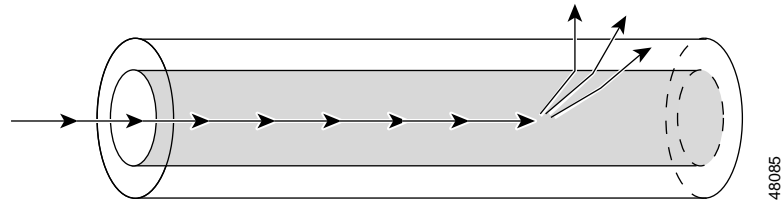
Figure 2-9 Rayleigh Scattering
