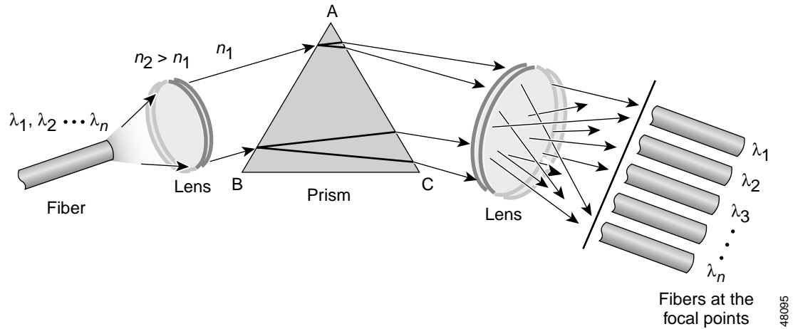
Figure 2-20 Prism Refraction Demultiplexing
