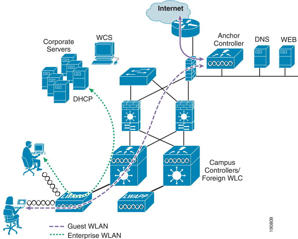
Figure 10-1 Centralized Controller Guest Access
