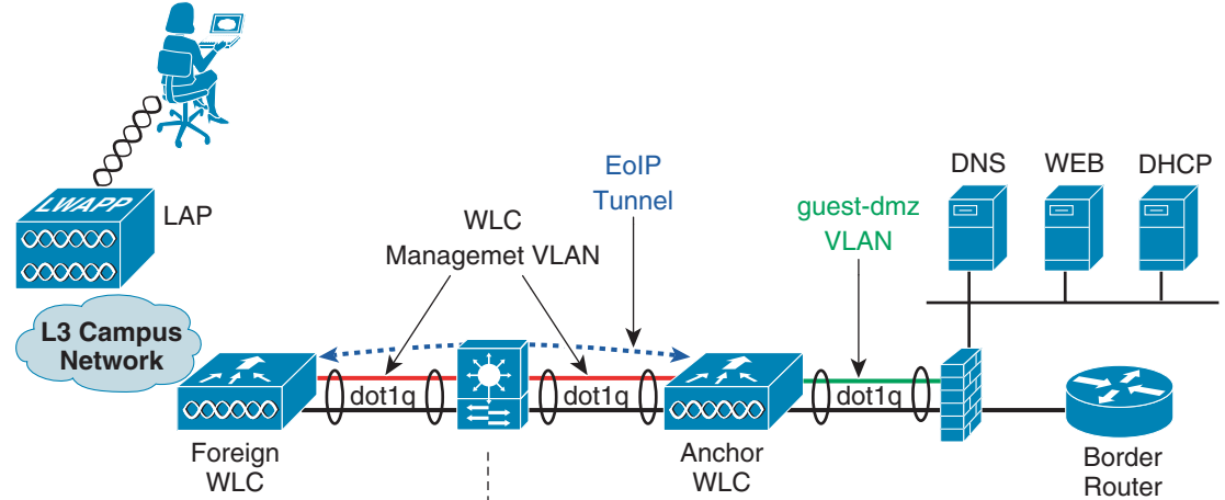
Figure 10-15 WLAN Configuration
