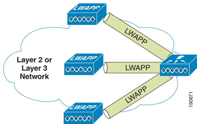
Figure 2-1 LWAPP APs Connected to a WLC
