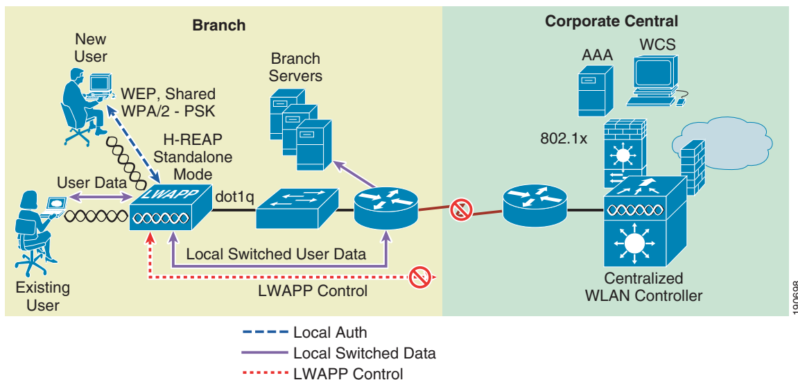
Figure 7-5 Authentication-Local/Switch-Local WLAN
