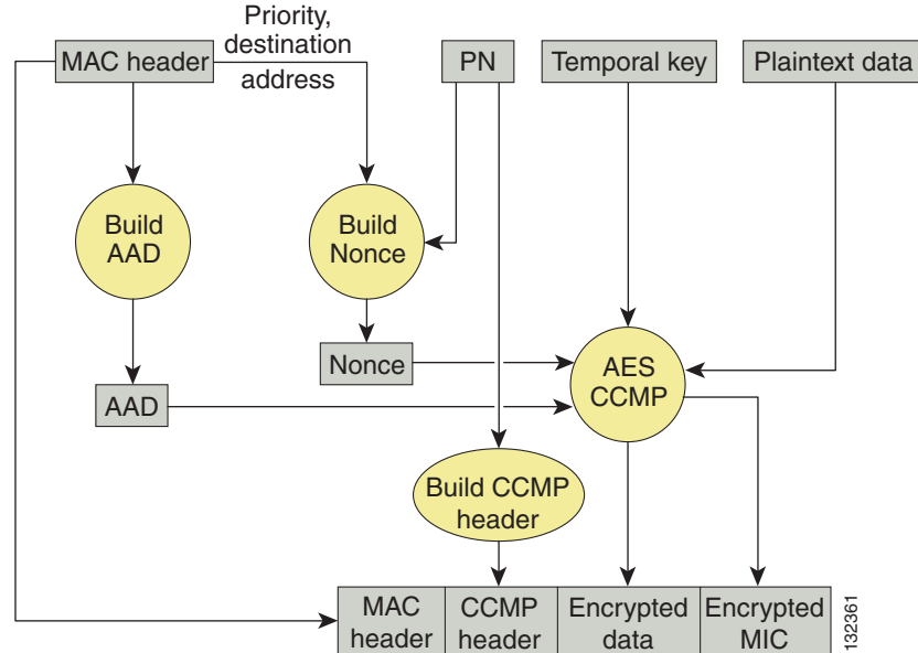
Figure 4-8 WPA2 AES CCMP
