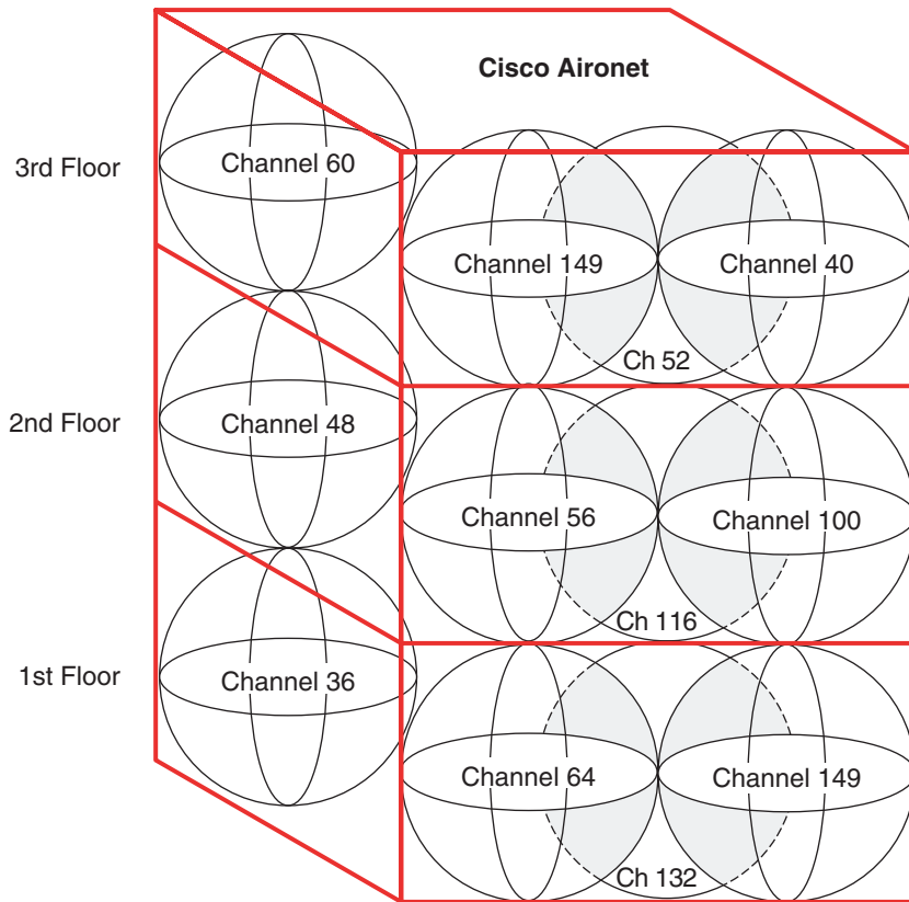
Figure 9-5 Vertical Channel Separation
