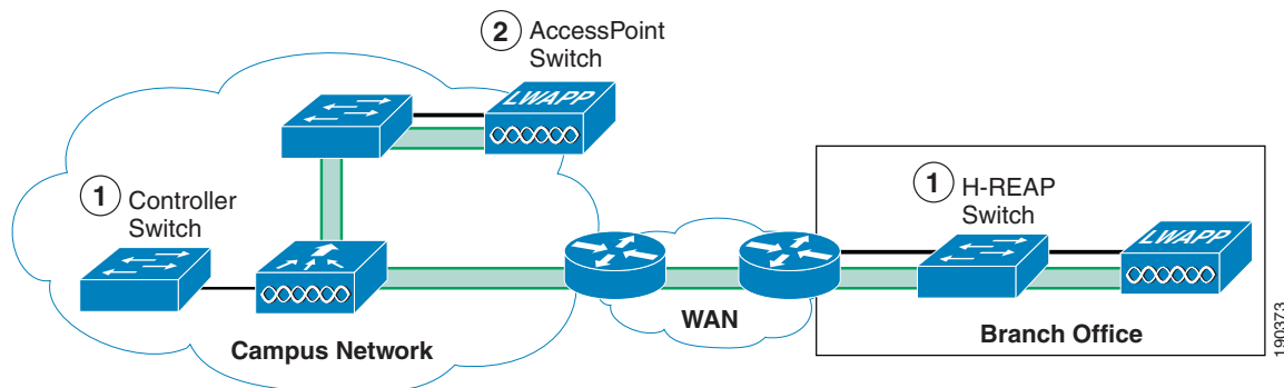
Figure 4-31 Access Switches
