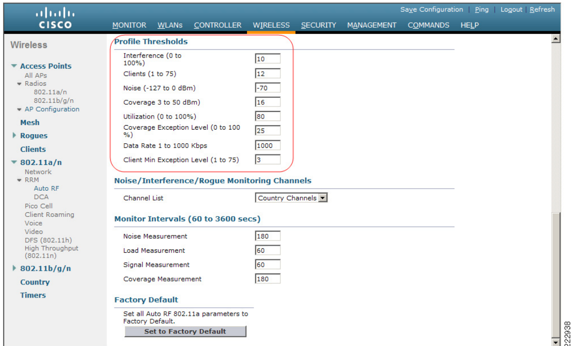
Figure 3-18 Auto-RF (Section 3)
