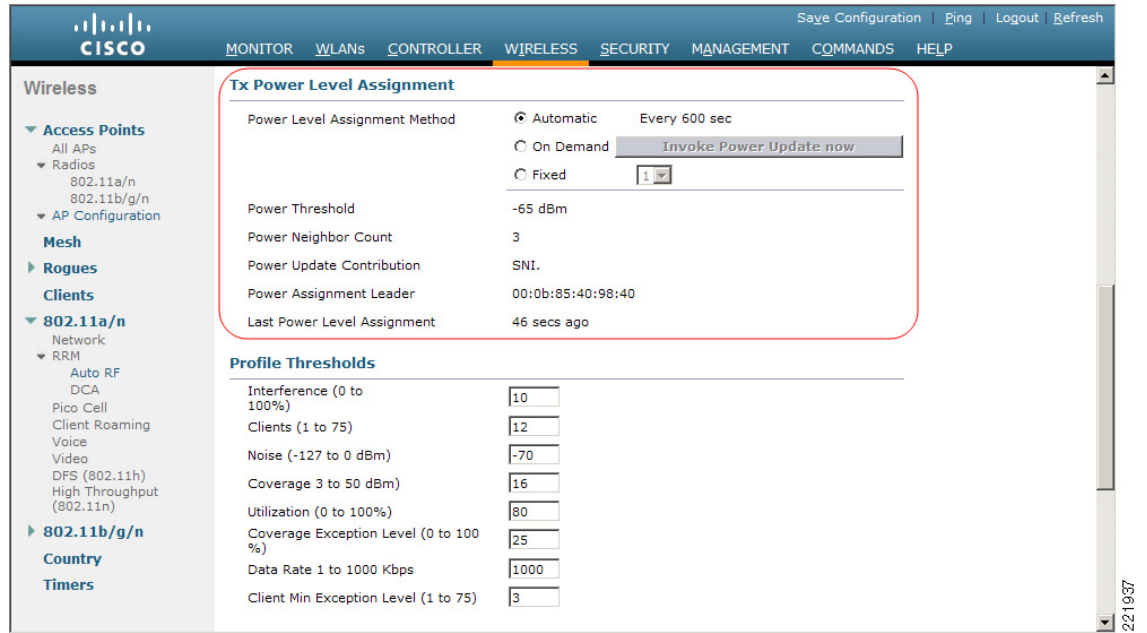
Figure 3-17 Auto-RF (Section 2)
