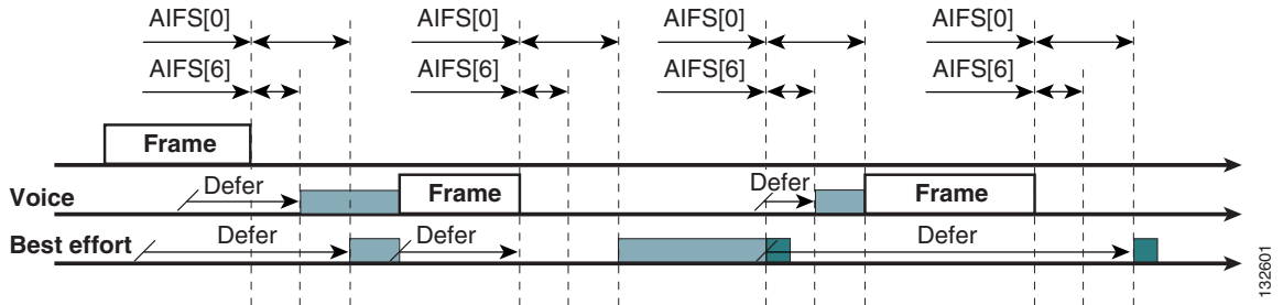
Figure 5-9 EDCA Example
