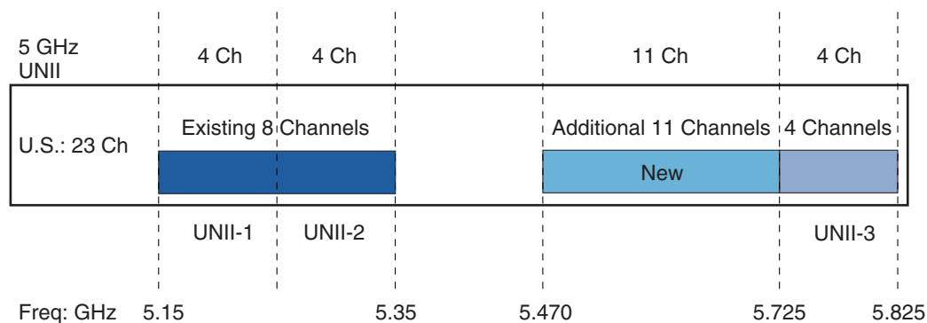
Figure 3-1 802.11 Channel Capacity
