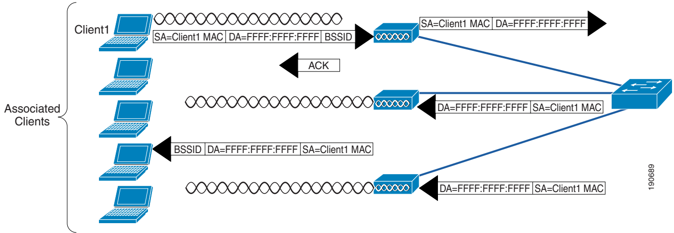
Figure 2-13 802.11 Broadcast/Multicast
