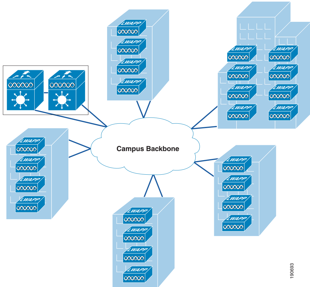
Figure 2-14 WLCs Centralized
