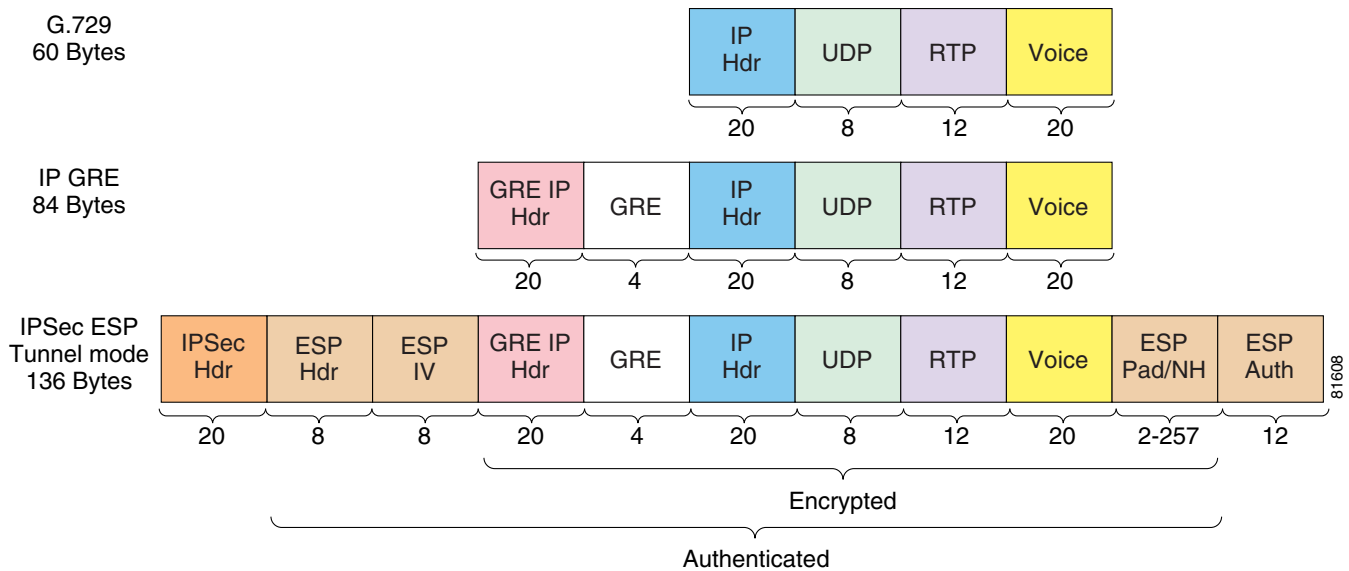
Figure 4-3 IPsec Encrypted G.729 Packet Anatomy
