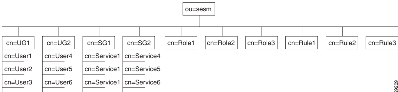
Figure 1-5 Directory Tree Structure for CDAT
